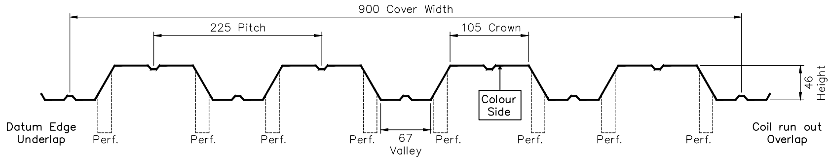
SECTION THROUGH PROFILE
