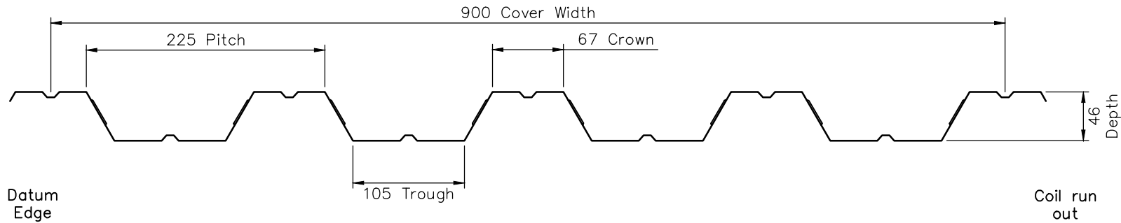
SECTION THROUGH PROFILE
