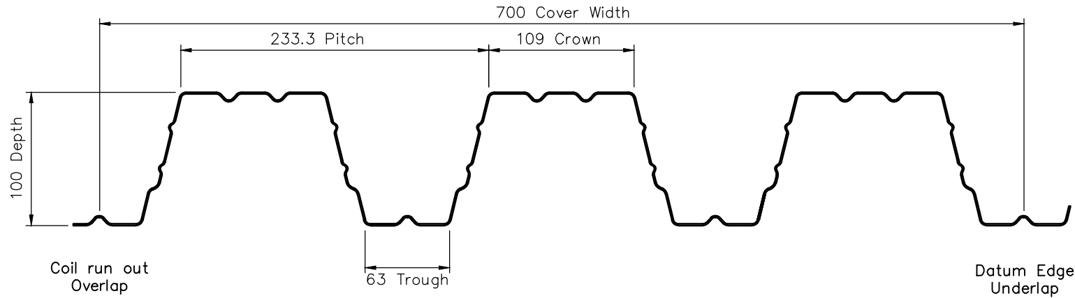
SECTION THROUGH PROFILE
